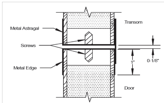
Square cut door and transom panel with metal edge and astragal
