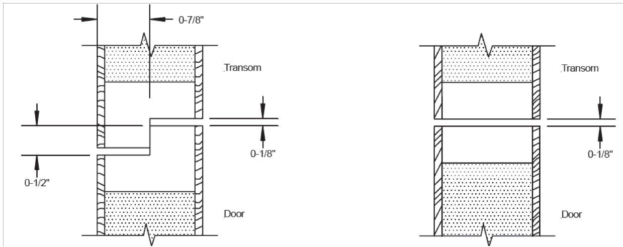
Square cut door and transom panel
