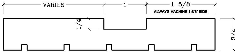
T-JAMB (NON-RATED) (1 3/8" DOOR)
